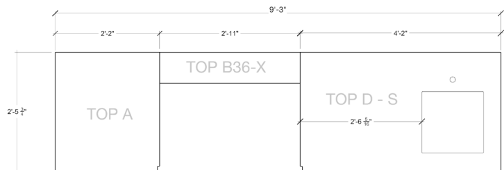
COUNTERTOP TEMPLATE
