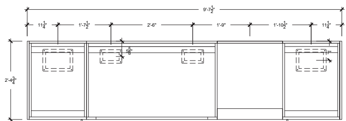
FRONT VIEW (Gas & Electrical Conduits Access Points)
