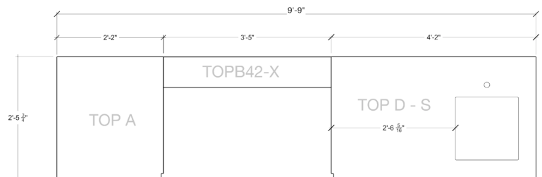
COUNTERTOP TEMPLATE
