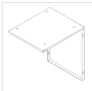
Grill Base Cabinet (38.5")
