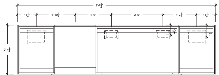
FRONT VIEW (Gas & Electrical Conduits Access Points)
