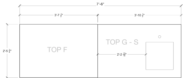
COUNTERTOP TEMPLATE
