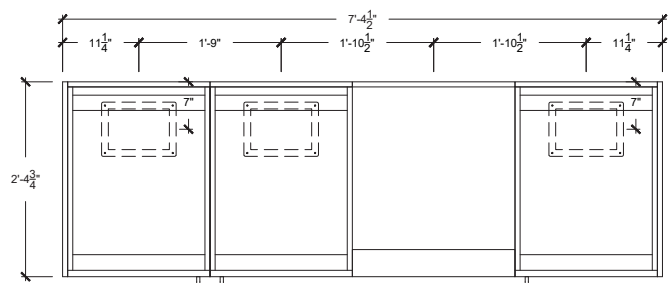
TOP VIEW (Gas & Electrical Conduits Access Points)
