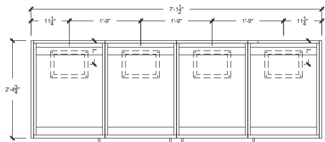
TOP VIEW (Gas & Electrical Conduits Access Points)
