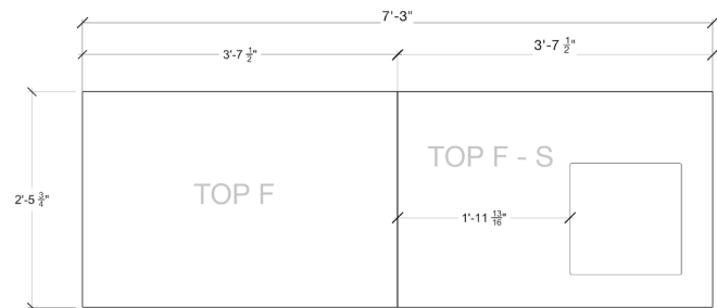
COUNTERTOP TEMPLATE
