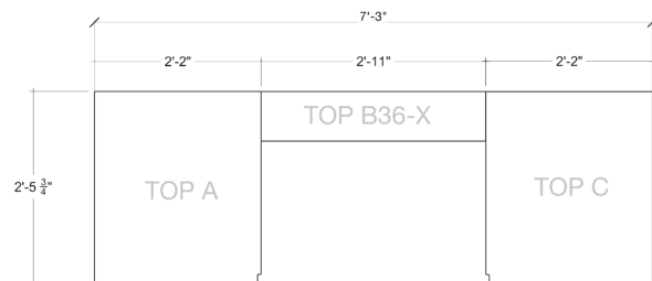
COUNTERTOP TEMPLATE
