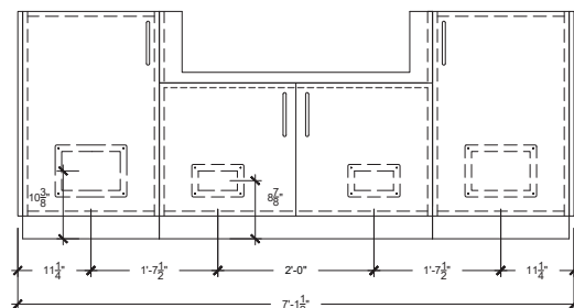
FRONT VIEW (Gas & Electrical Conduits Access Points)
