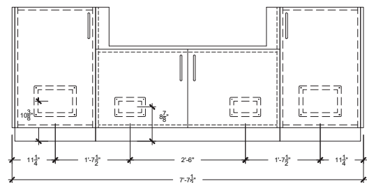
FRONT VIEW (Gas & Electrical Conduits Access Points)
