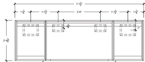
TOP VIEW (Gas & Electrical Conduits Access Points)
