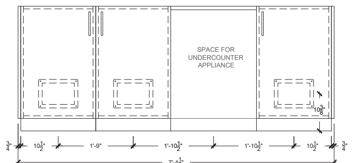
FRONT VIEW (Gas & Electrical Conduits Access Points)
